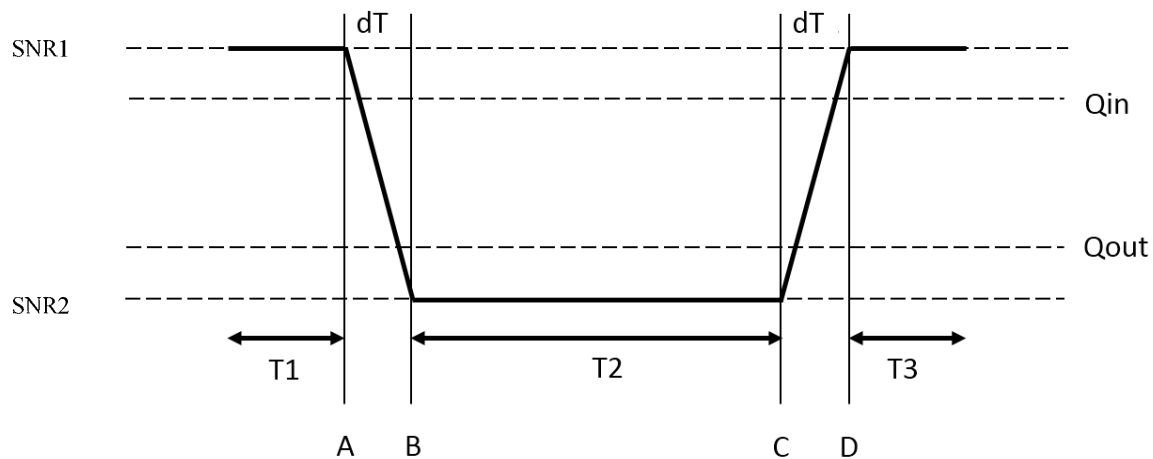
Figure A.7.3.93.1-1: SNR variation for in-sync testing without DRX
