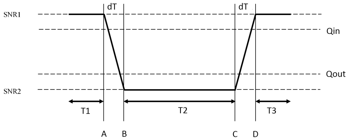
Figure A.7.3.91.1-1: SNR variation for in-sync testing with DRX
