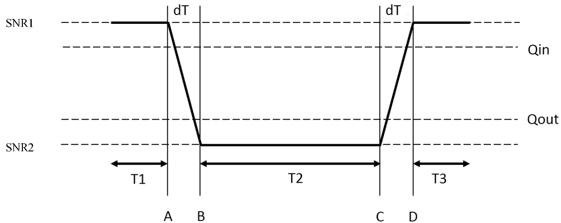
Figure A.7.3.90.1-1: SNR variation for in-sync testing with DRX
