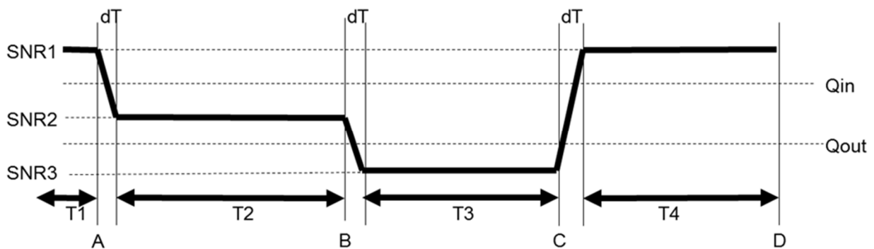
Figure A.7.3.94.1-1: SNR variation for out-of-sync testing
