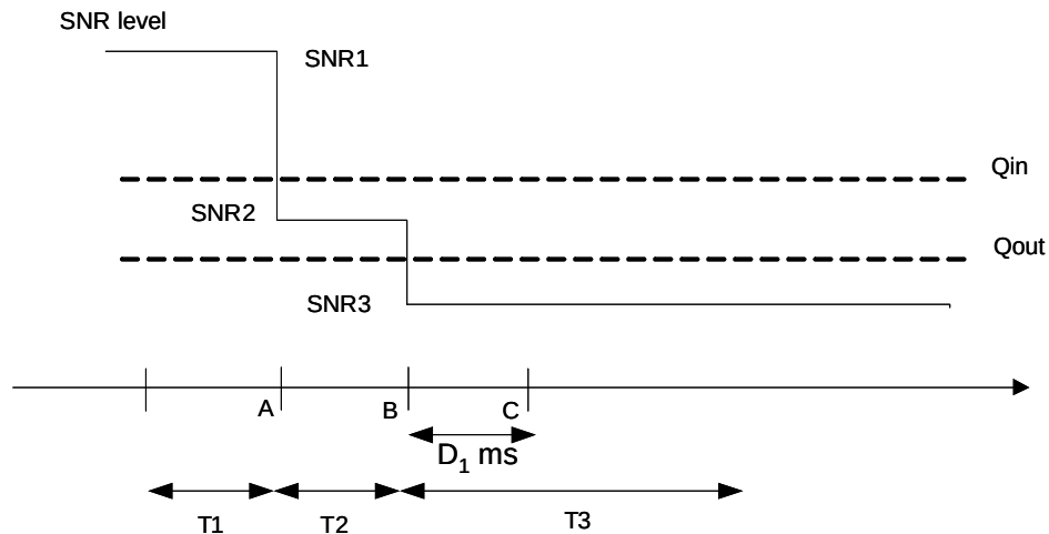
Figure A.7.3.76.1-1: SNR variation for out-of-sync testing in DRX
