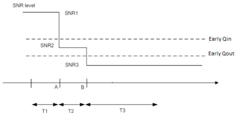
Figure A.7.3.84.1-1: SNR variation for early out-of-sync testing
