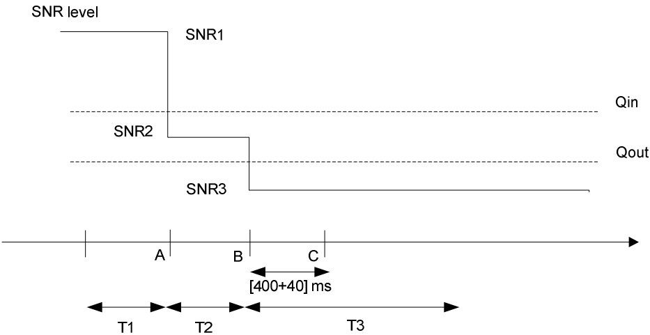
Figure A.7.3.74.1-1: SNR variation for out-of-sync testing
