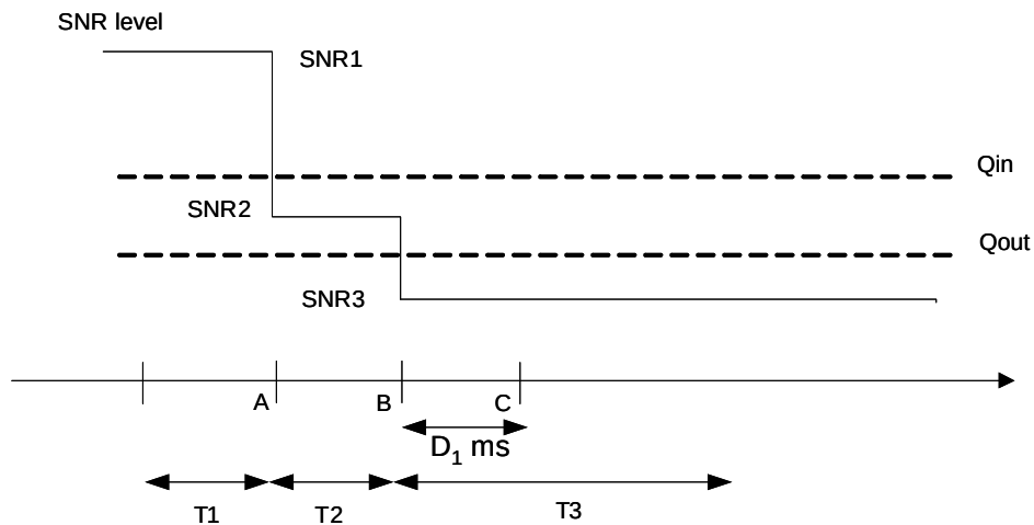
Figure A.7.3.80.1-1: SNR variation for out-of-sync testing in DRX
