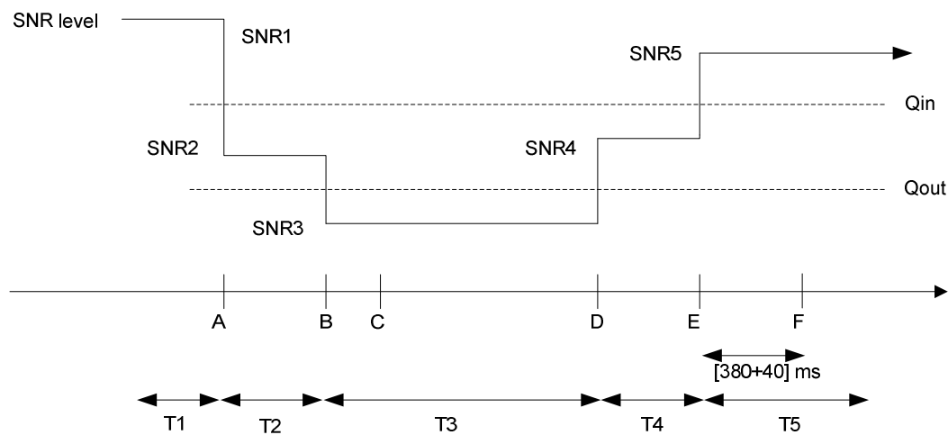
Figure A.7.3.2.1-1 SNR variation for in-sync testing
