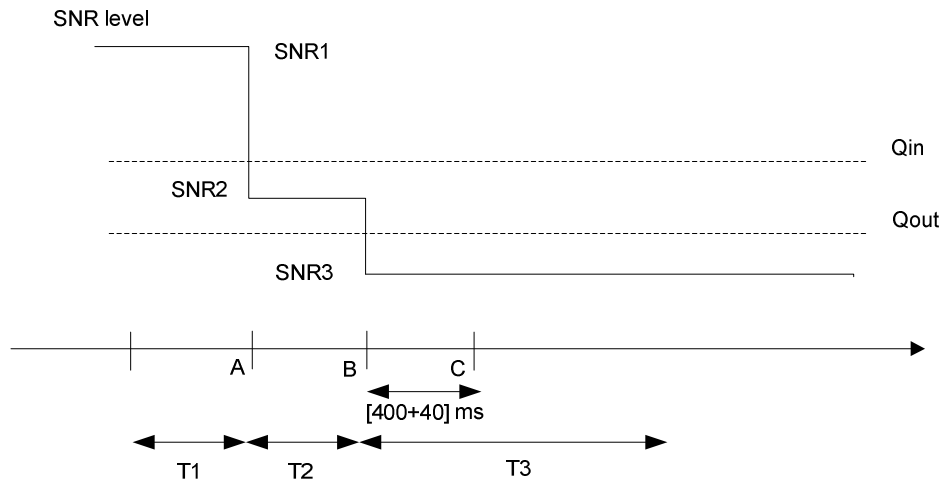
Figure A.7.3.78.1-1: SNR variation for out-of-sync testing
