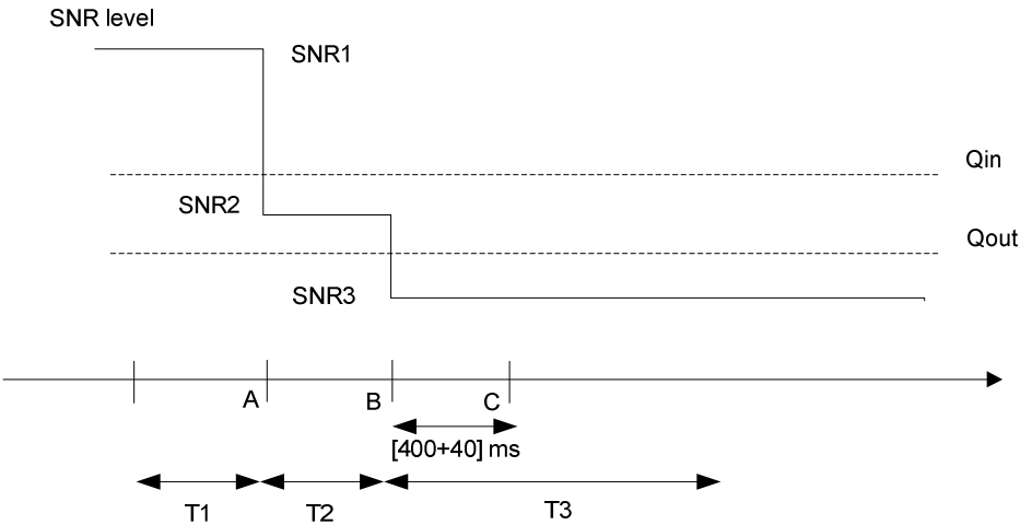
Figure A.7.3.52.1-1: SNR variation for out-of-sync testing
