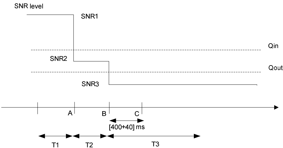
Figure A.7.3.52.1-1: SNR variation for out-of-sync testing
