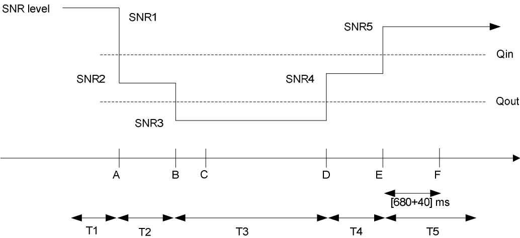
Figure A.7.3.75.1-1: SNR variation for in-sync testing
