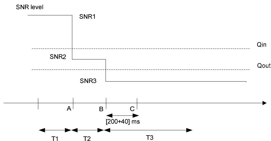
Figure A.7.3.13.1-1 SNR variation for out-of-sync testing
