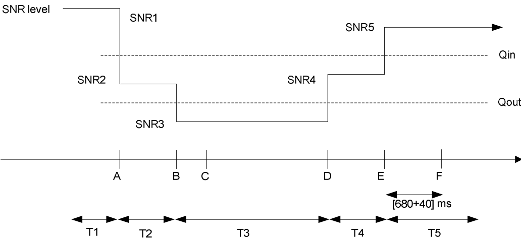
A.7.3.57.1-1: SNR variation for in-sync testing
