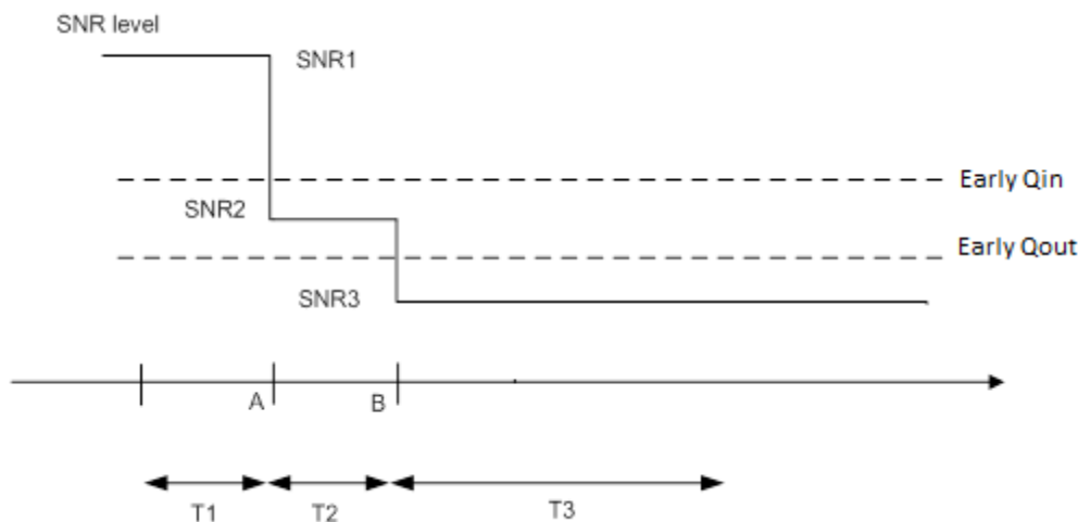
Figure A.7.3.70.1-1: SNR variation for early out-of-sync testing
