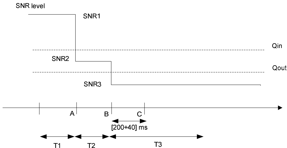
Figure A.7.3.26.1-1: SNR variation for out-of-sync testing
