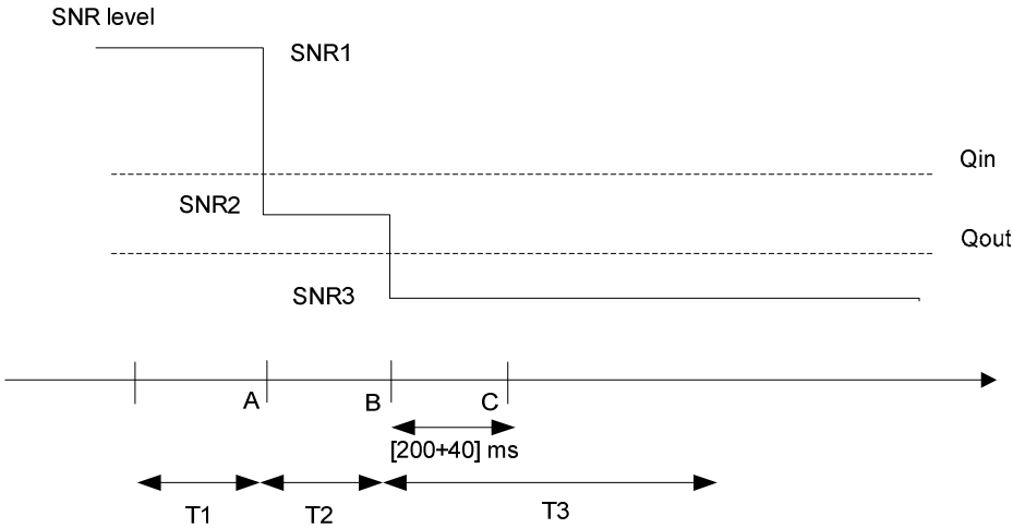
Figure A.7.3.9.1-1 SNR variation for out-of-sync testing
