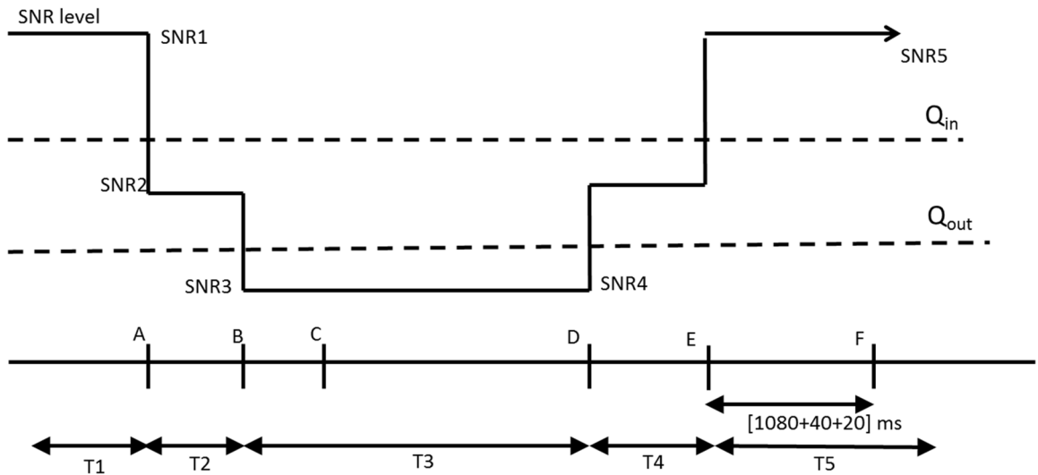
Figure A.7.3.55.1-1: SNR variation for in-sync testing in DRX
