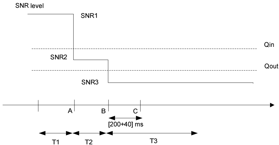
Figure A.7.3.18.1-1 SNR variation for out-of-sync testing
