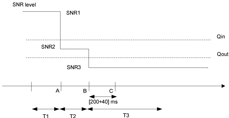
Figure A.7.3.17.1-1 SNR variation for out-of-sync testing
