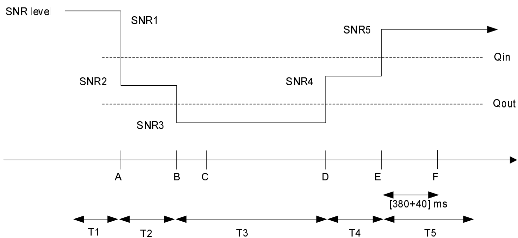
Figure A.7.3.31.1-1: SNR variation for in-sync testing
