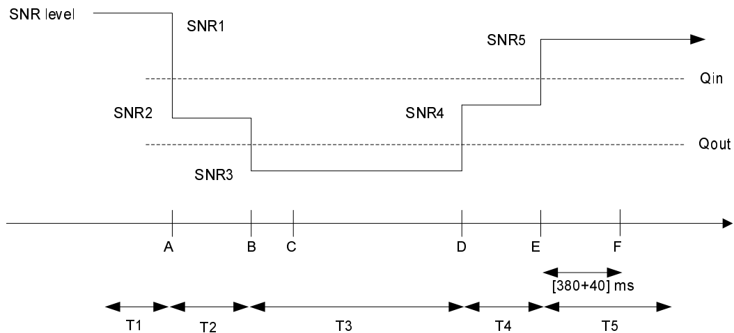
Figure A.7.35.1-1: SNR variation for in-sync testing
