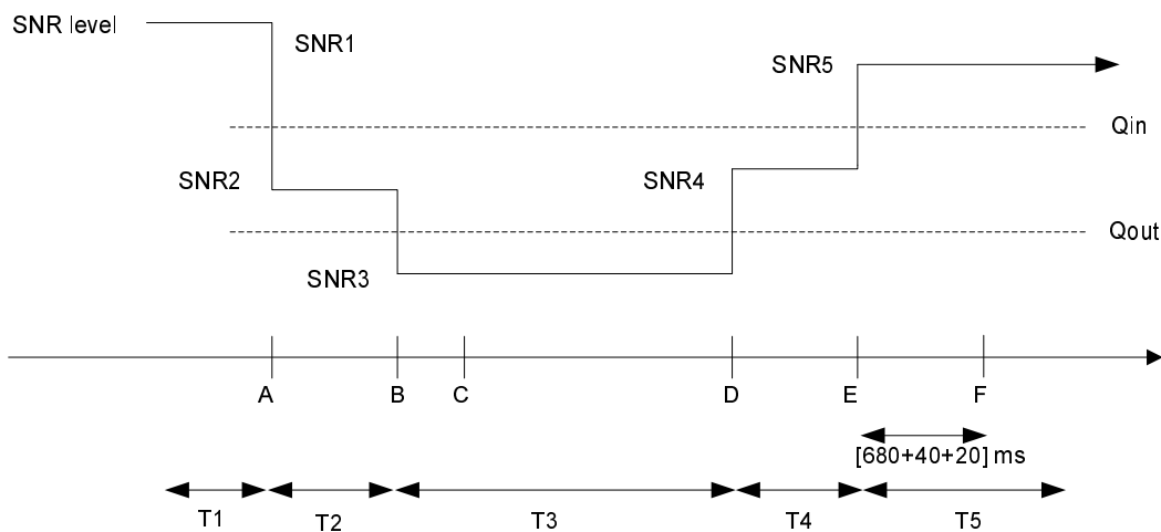
A.7.3.53.1-1: SNR variation for in-sync testing
