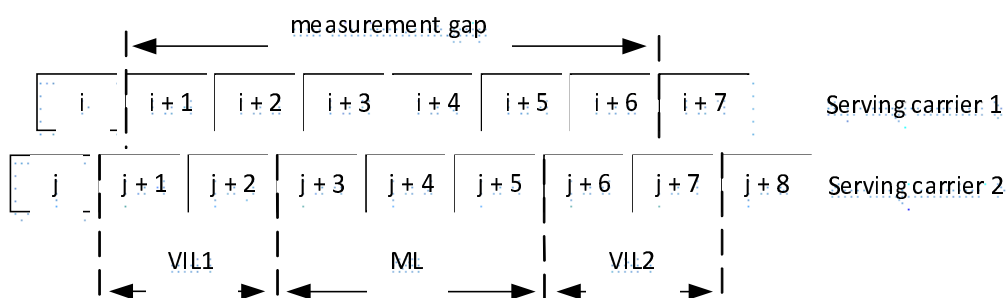
Figure 8.1.2.1.2-2: Measurement GAP and NCSG for dual connectivity
