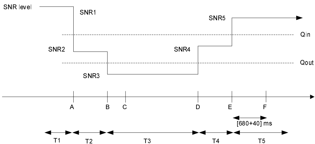
Figure A.7.3.49.1-1: SNR variation for in-sync testing
