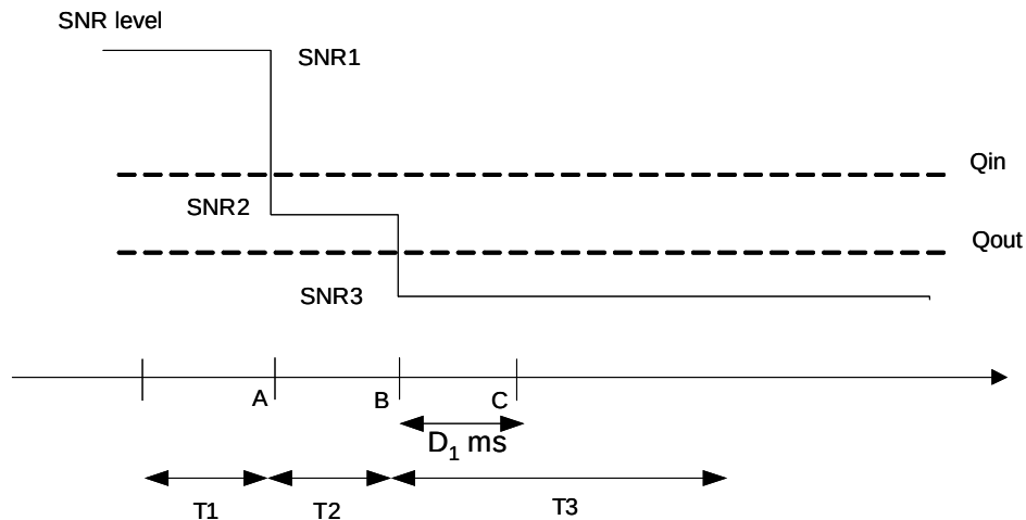
Figure A.7.3.32.1-1: SNR variation for out-of-sync testing in DRX
