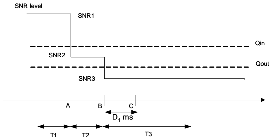
Figure A.7.3.7.1-5 SNR variation for out-of-sync testing in DRX
