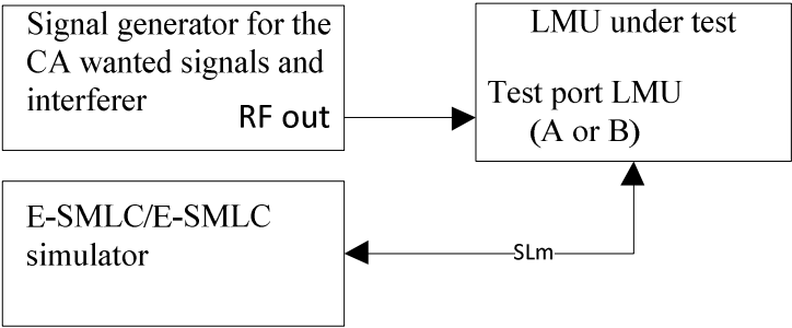
Figure G.3.2-1 Measuring system setup for UL RTOA measurement accuracy for LMU with CA
