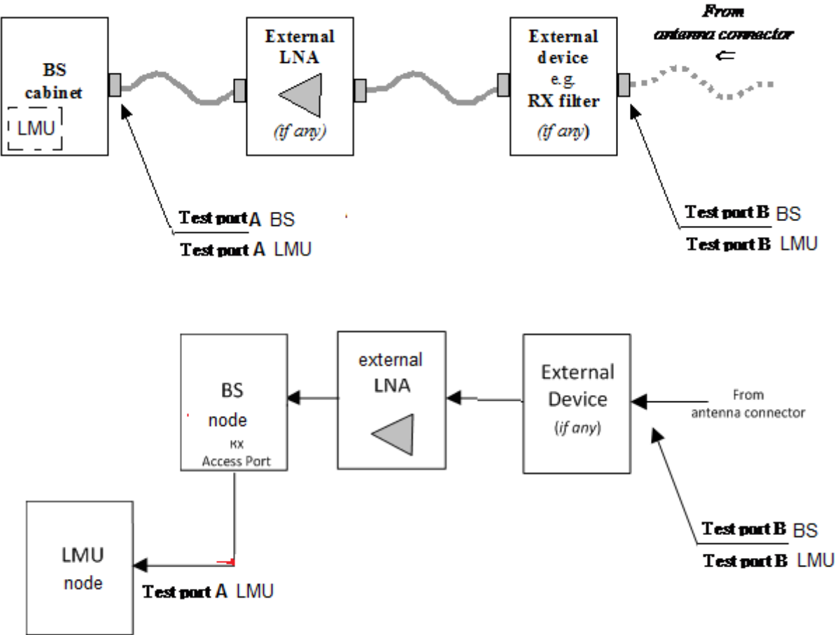
Figure 4.5-1: Two examples of receiver test ports for LMU class 1.
