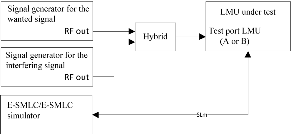
Figure G.1.4-1 Measuring system setup for LMU Adjacent channel selectivity and narrow-band blocking
