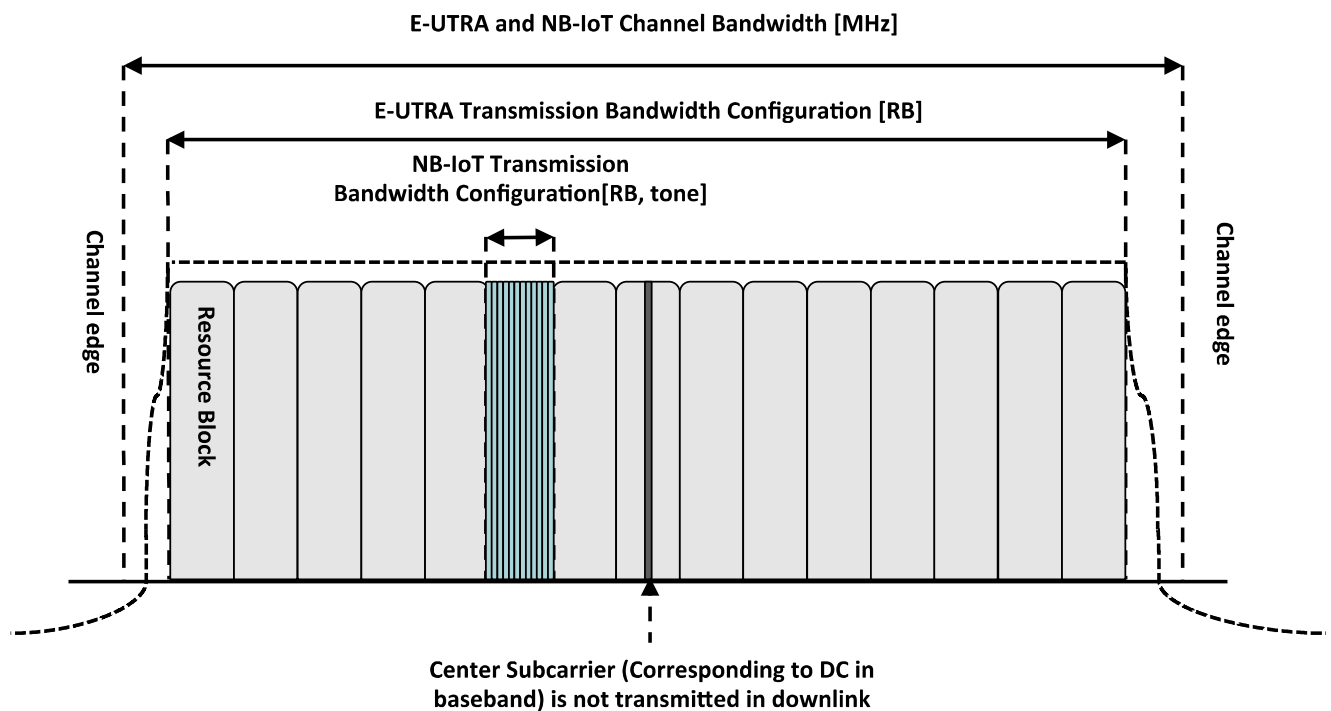
Figure 5.6-5 Definition of Channel Bandwidth and Transmission Bandwidth Configuration for NB-IoT in-band operation
