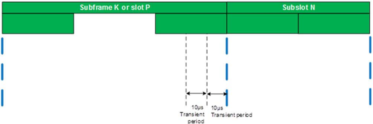
Figure 6.3.4.10-3: subframe TTI and subslot TTI boundary
