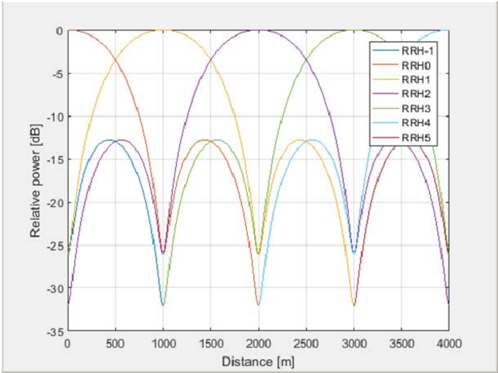
Figure B.3A-2 Ralative power level trajectories
