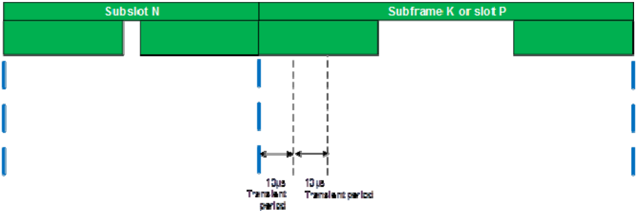
Figure 6.3.4.9-1: subslot TTI and subframe TTI boundary
