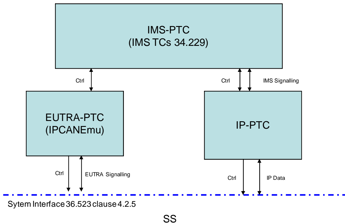
Figure 4: Extension to the Test Model to support 36.523-3 SS interface
