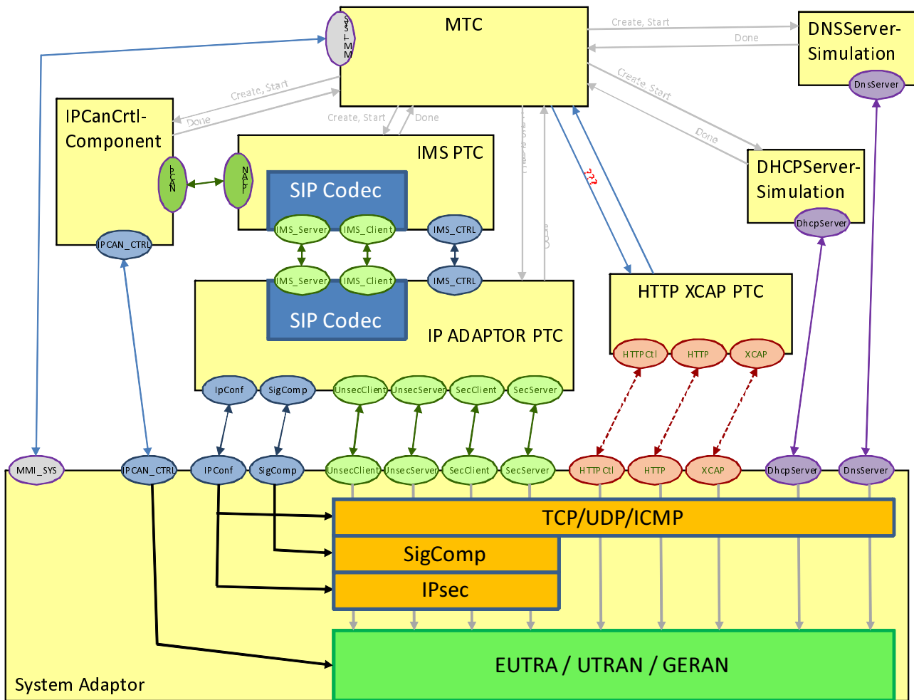
Figure 2: IMS CC test mode
