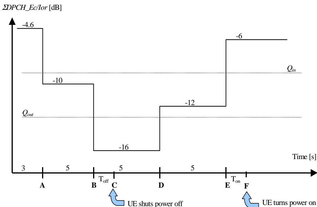
Figure 5.4.5.1: Test case for out-of-synch handling in the UE continuous transmission
