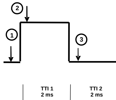
Figure 5.2ED.1: Transmit power profile showing measurement points
