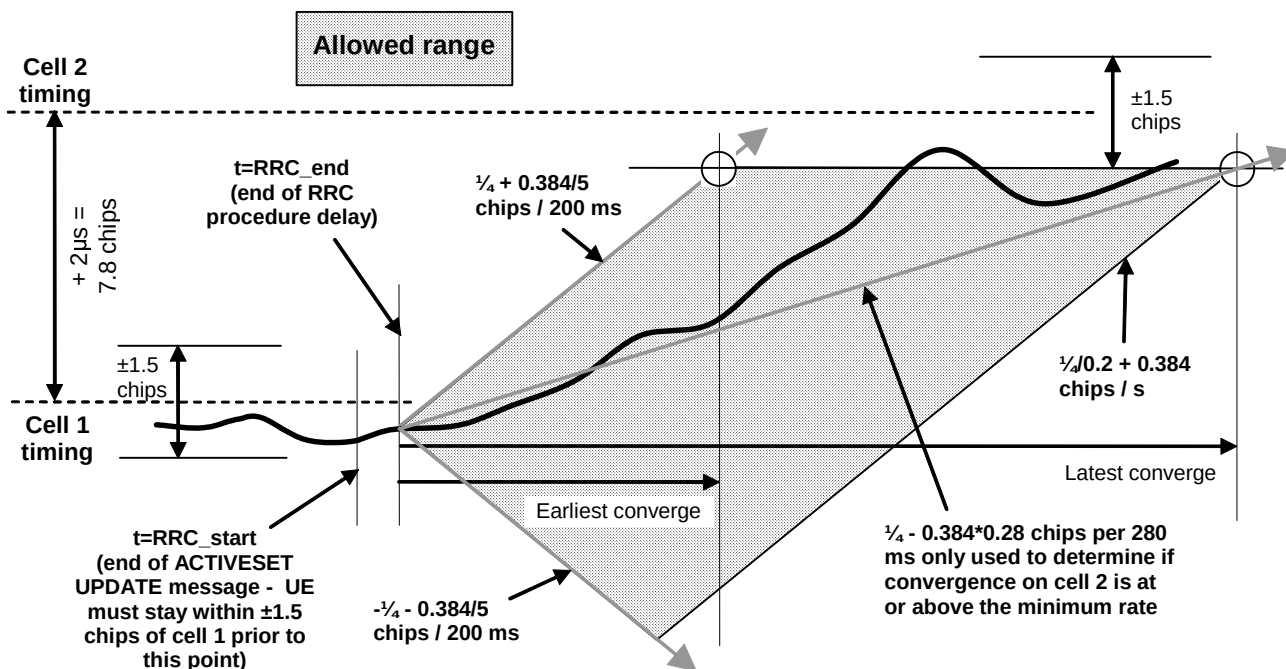
Figure 8.5.1.5 Illustration of measurement principle (excluding measurement uncertainty)
