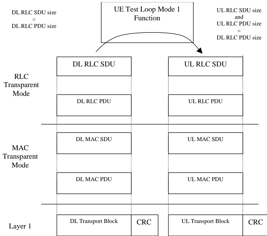
Figure A.2.2. Example of a configuration used for BER measurement
