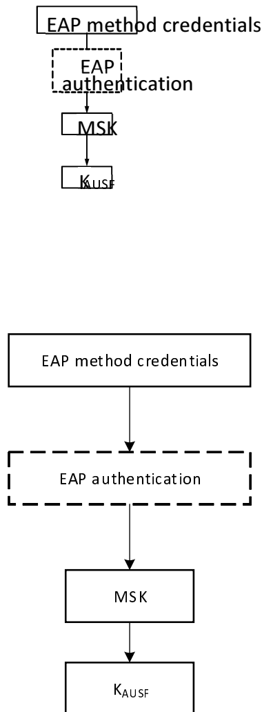
Figure I.2.3.2-1: K_{\text{AUSF}} derivation for primary authentication towards an external Credentials holder using AAA server
