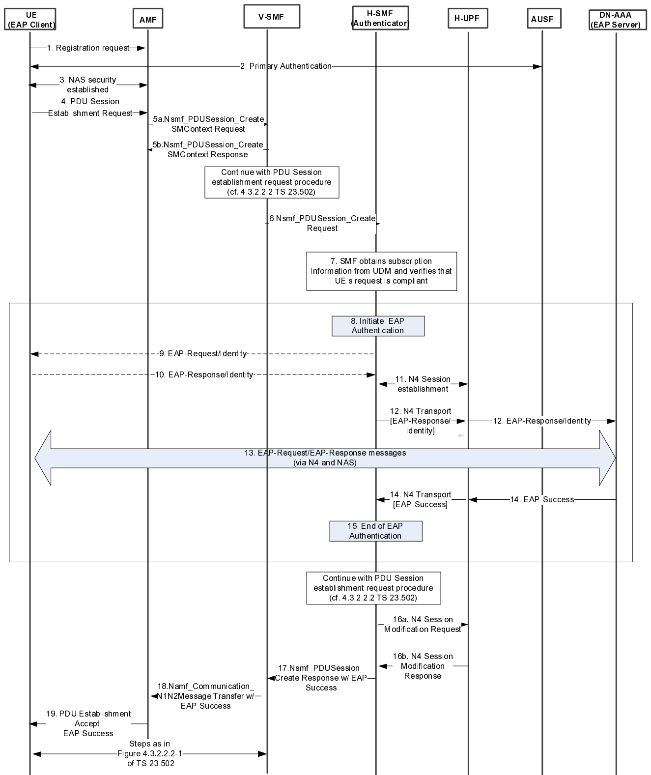
Figure 11.1.2-1: Initial EAP Authentication with an external AAA server
