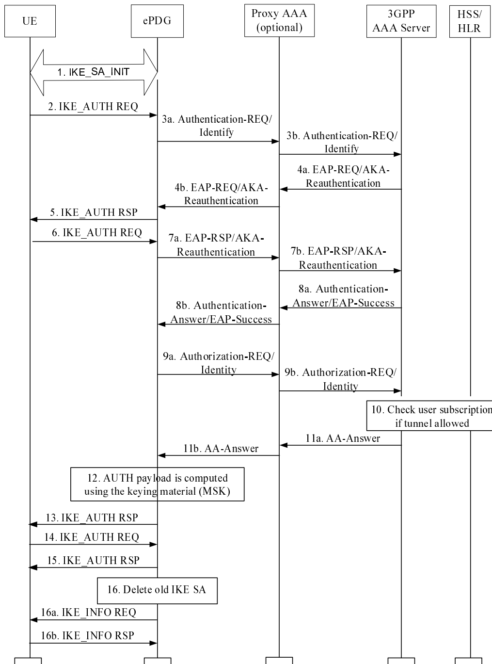
Figure 8.2.3-1: Untrusted Tunnel - Fast Re-authentication
