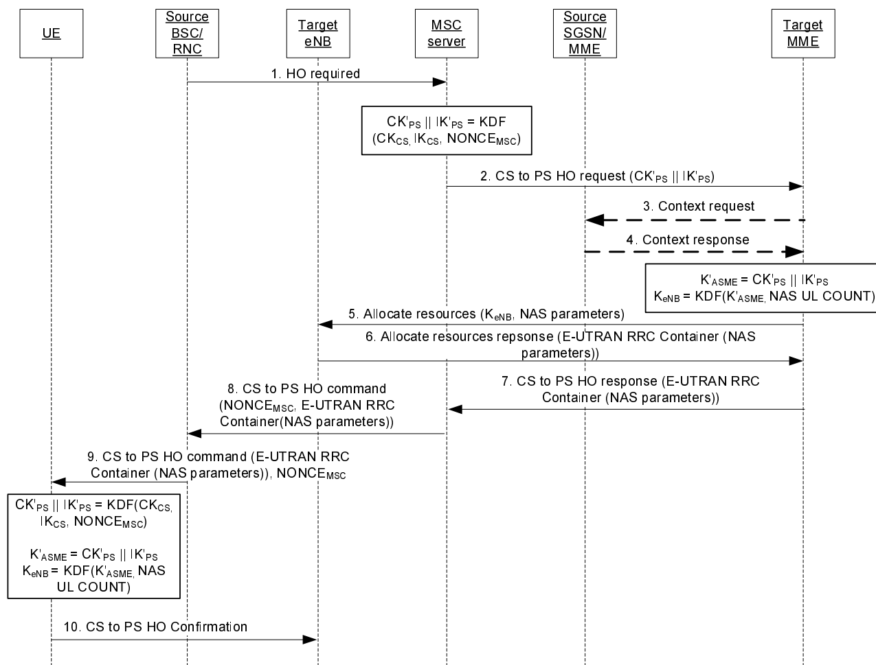
Figure 14.3.1-1: SRVCC handover from UTRAN/GERAN to E-UTRAN. Key derivations in the figure are only shown for UMTS subscribers.
