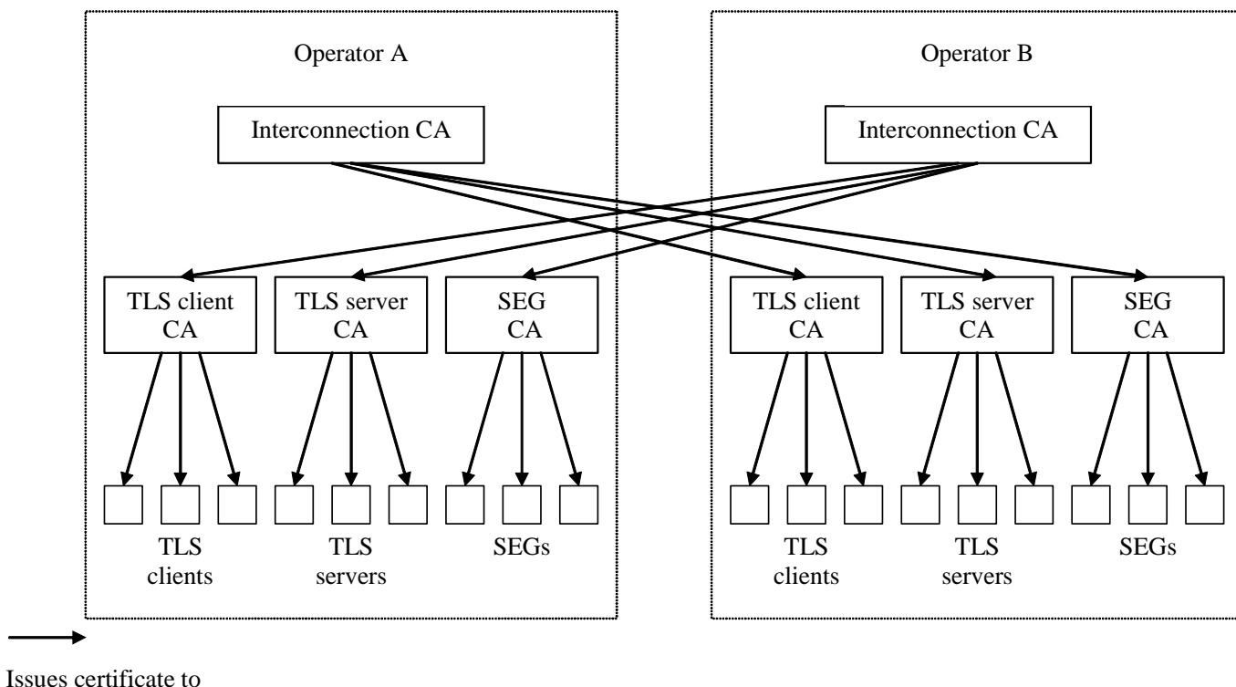
Figure 3: Certificate Hierarchy
