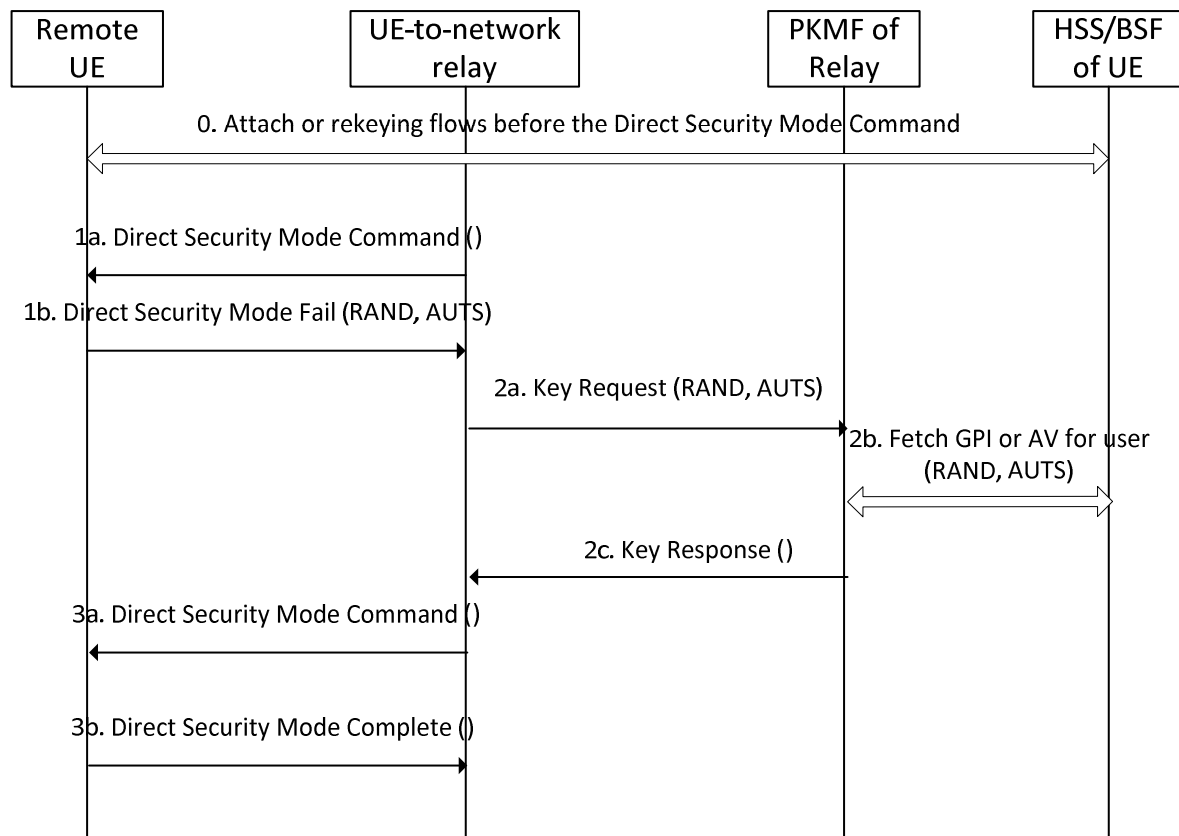
Figure 6. 7.3.2.1.2-1: Re-synchronisation flows
