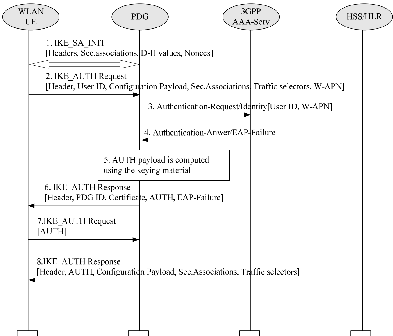
Figure 7AA: Skipping authentication for IMS emergency call
