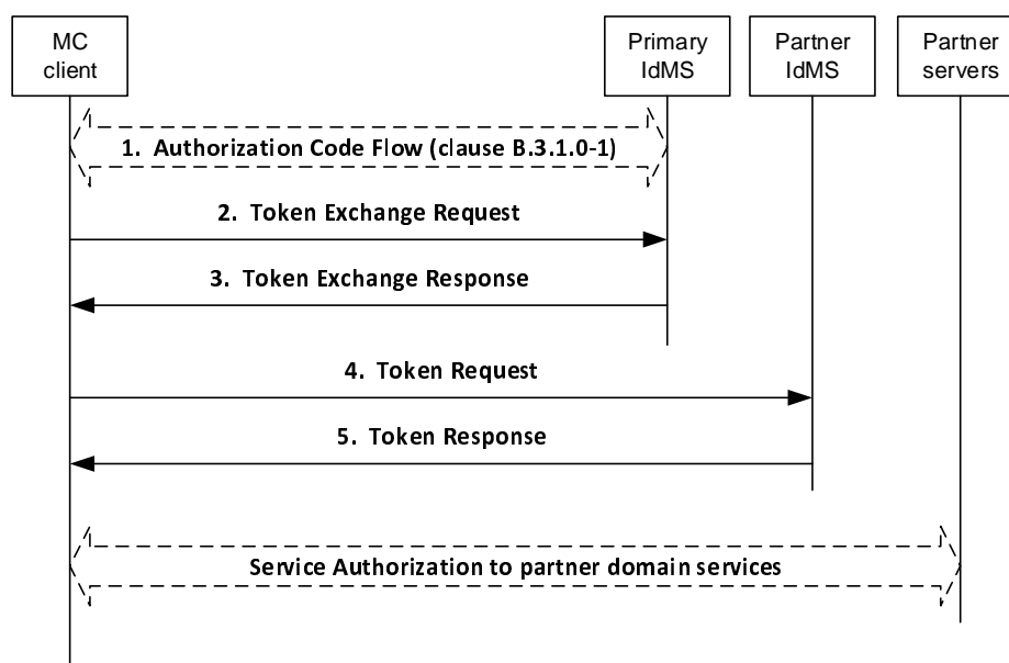
Figure 5.1.4.2-2: Token exchange procedure
