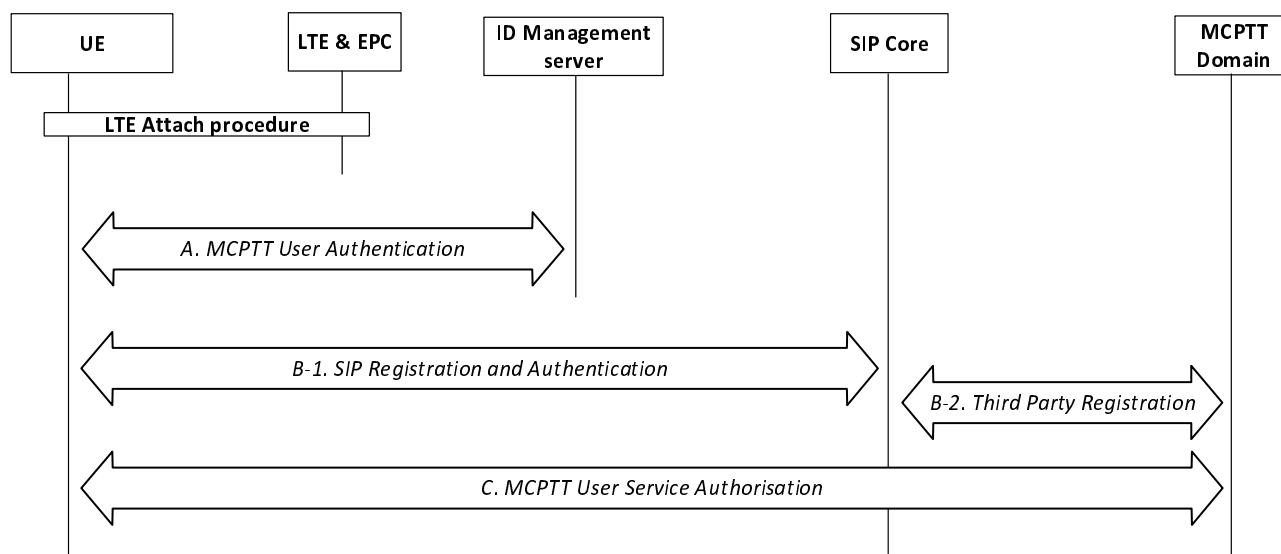
Figure 5.1-1: MCPTT Authentication
