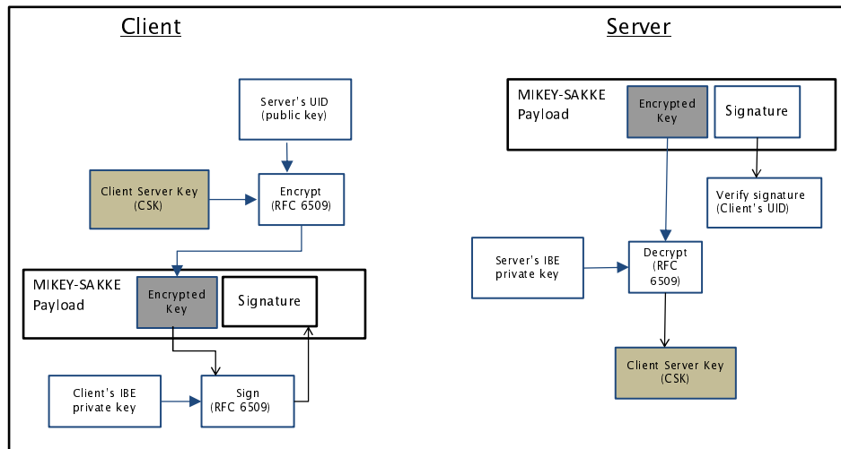
Figure 9.1.3.4-1: Functional diagram for Identity based distribution of CSK
