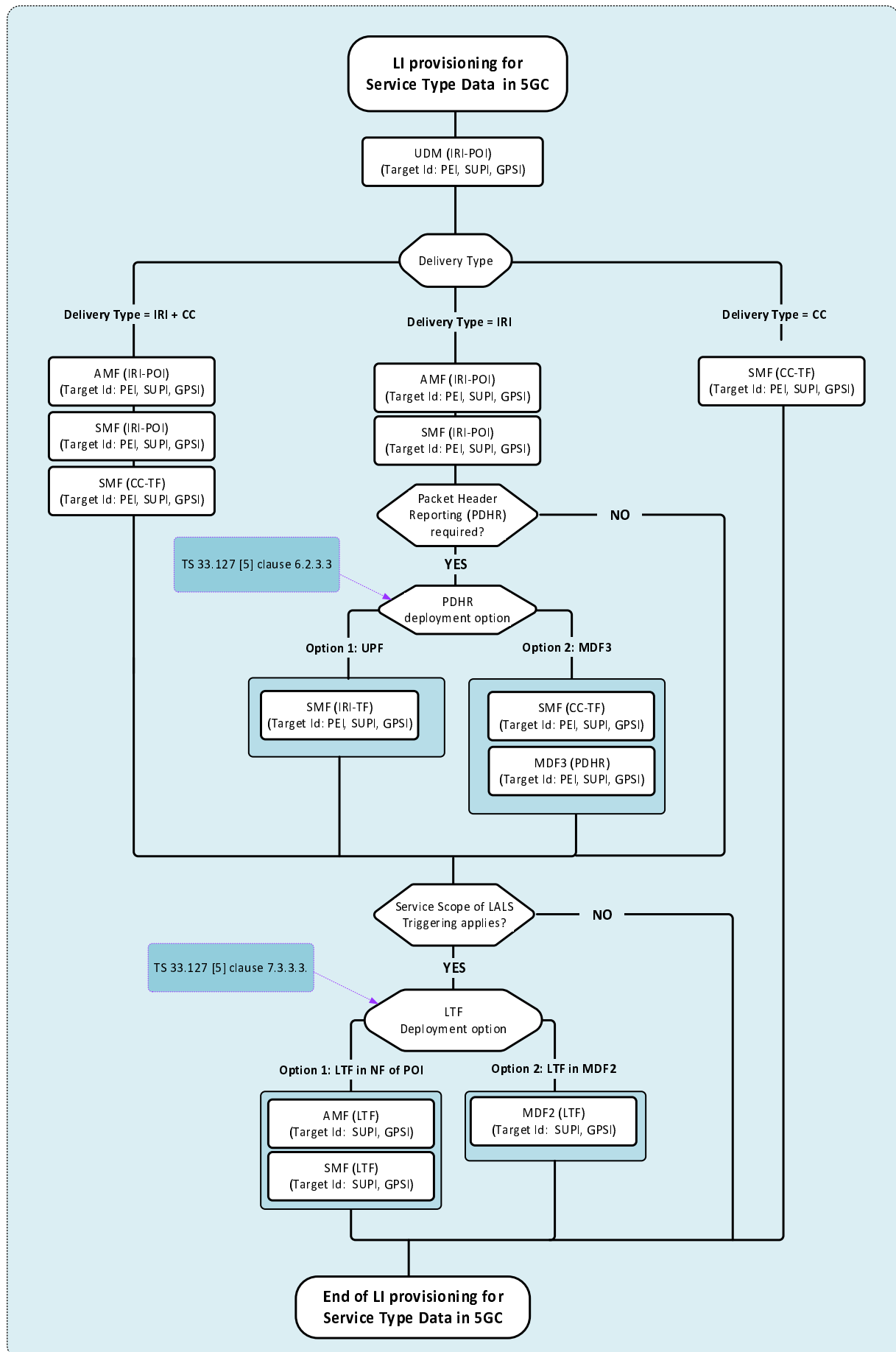
Figure G.4-2: LIPF logic for the service type Data in 5GC
