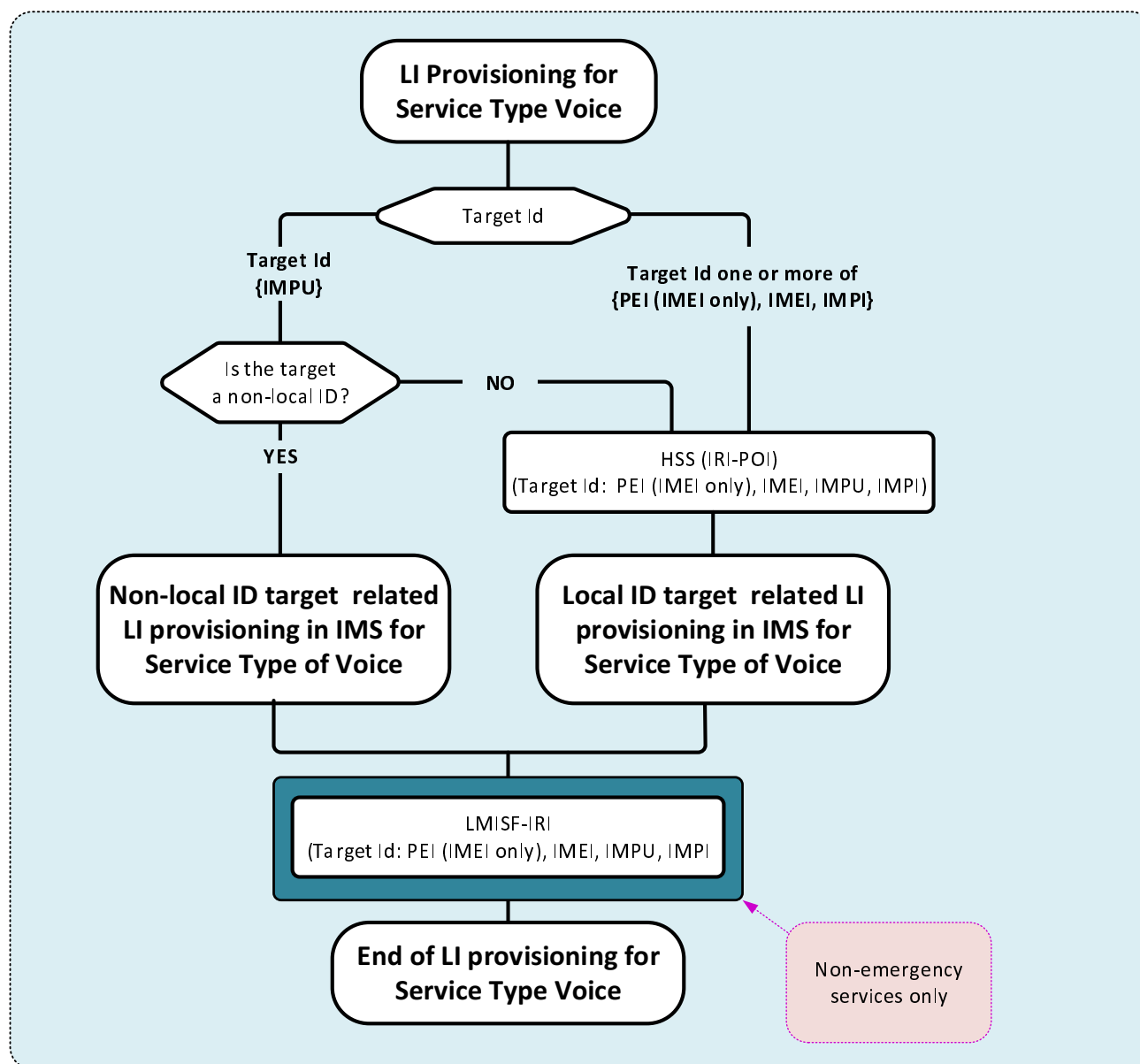
Figure G.5-2: Top level view of LIPF logic for service type of Voice
