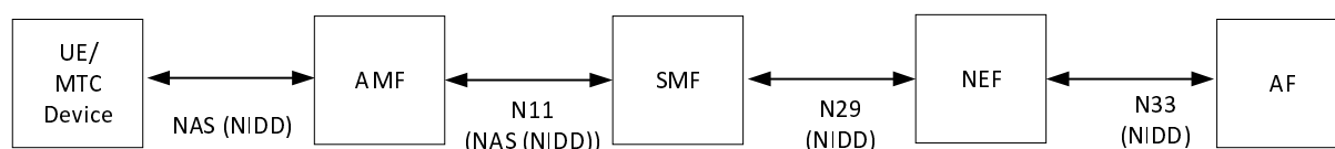
Figure 7.8.1.2.1-1: 5GS Architecture for NIDD using NEF
