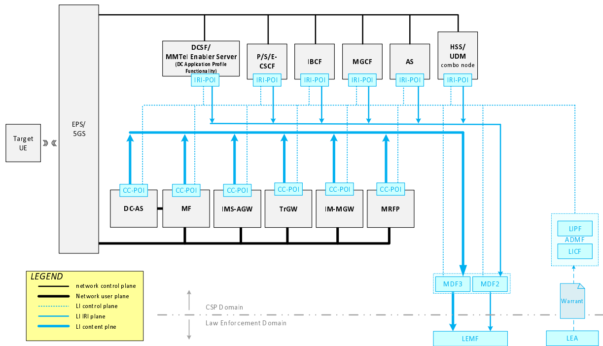
Figure 7.4.1-1: EPS/5GS-Anchored IMS High Level LI Architecture
