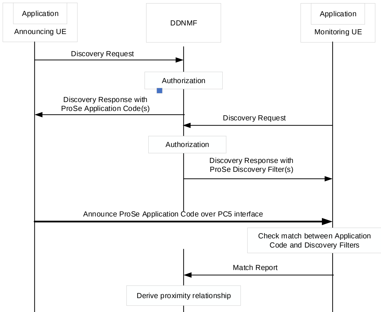
Figure G.2.1-1: High level Direct Discovery procedure
