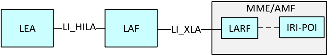
Figure 7.3.5.2.1-1: Delivery of the retrieved information via the LI_HILA
