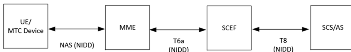
Figure 7.10.1.2.1-1: EPS Architecture for NIDD using SCEF
