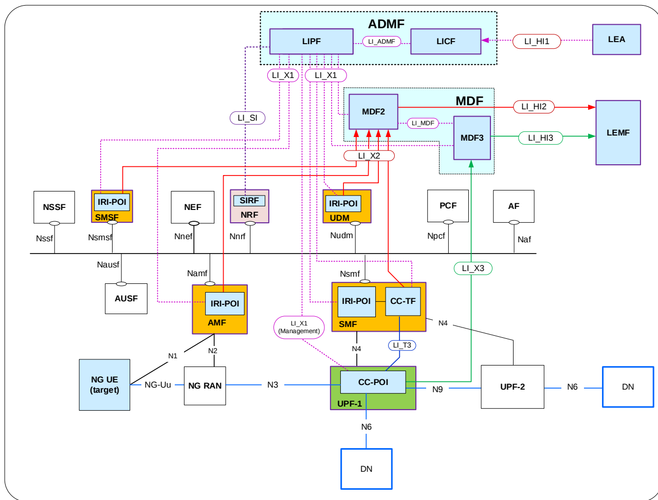
Figure A.3.2-1: Network topology showing CC-POI at one UPF
