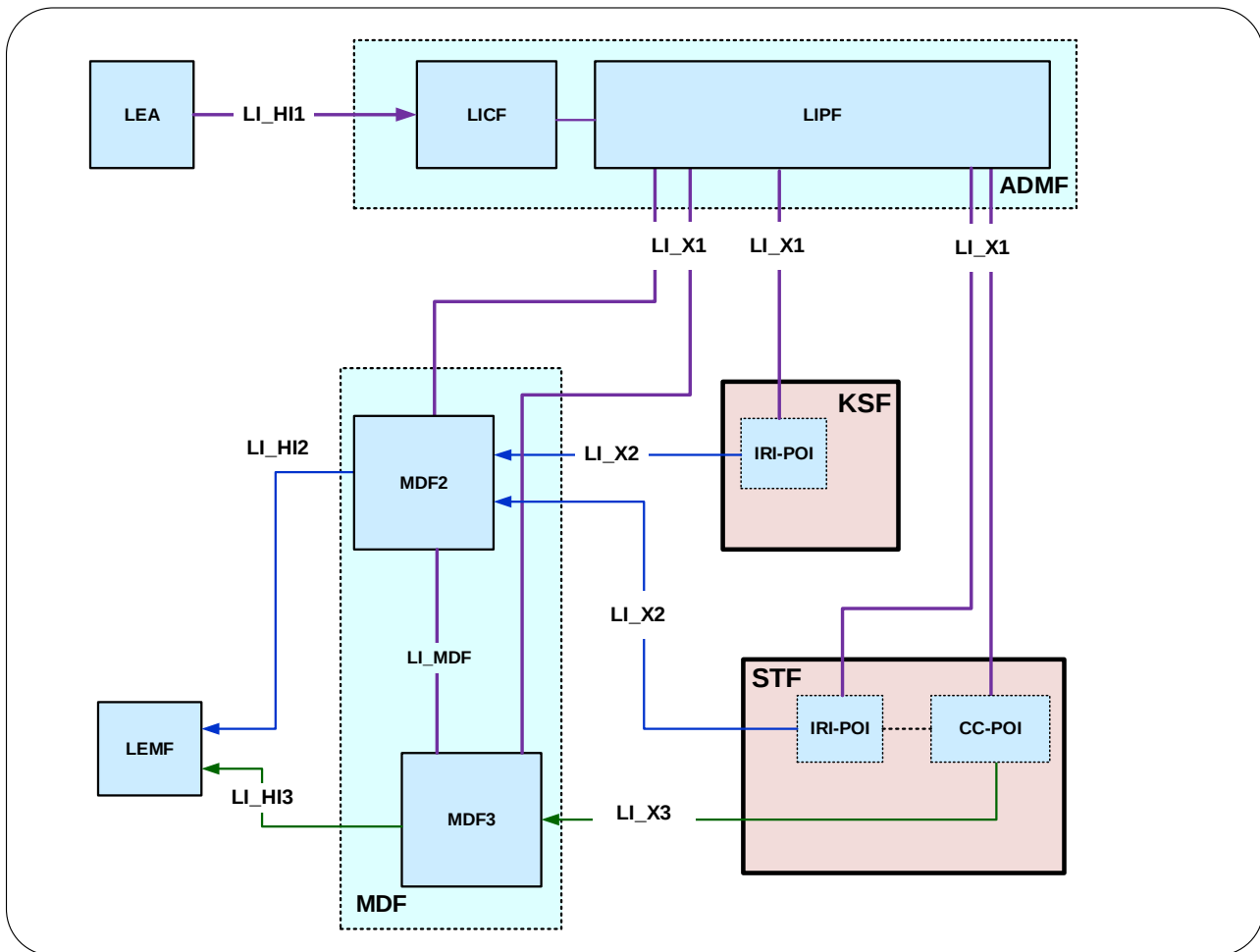
Figure 7.15.2-1: General architecture, STF using 5G native identifiers.
