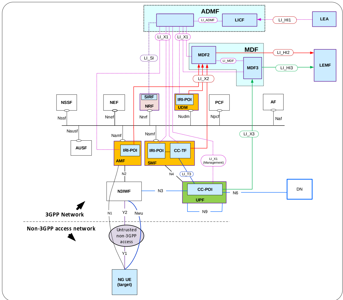
Figure A.4.2-1: Network topology showing LI for non-3GPP access to 5G via N3IWF
