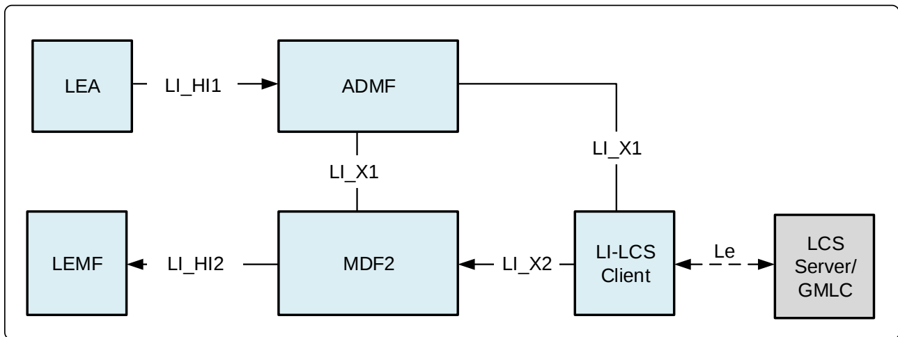
Figure 7.3.3.2.1-1: LALS model for target positioning
