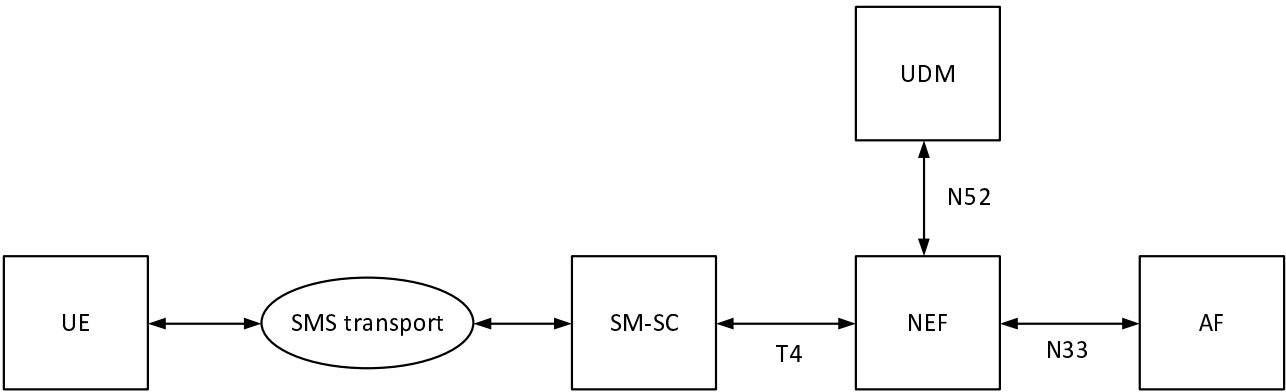
Figure 7.9.3.1-1: 5GS architecture for device triggering
