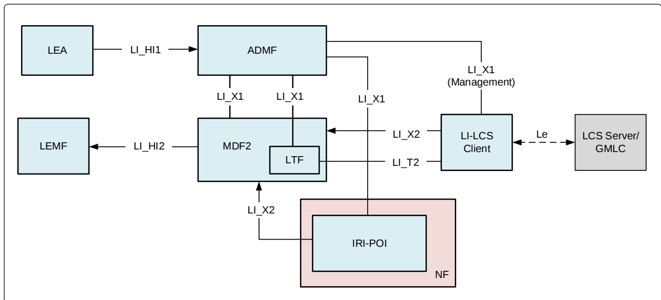
Figure 7.3.3-2: LALS Model for triggered location (MDF/LTF option)
