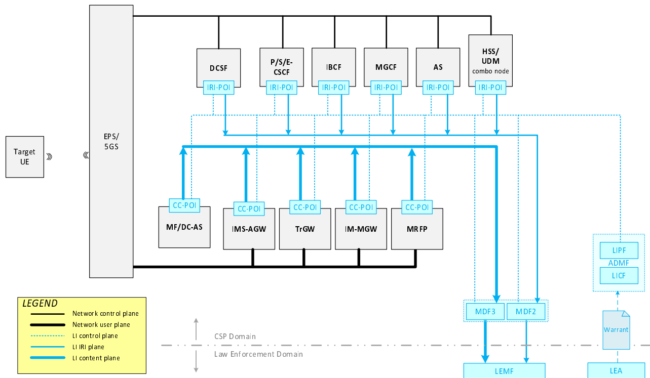
Figure 7.4-1: EPS/5GS-Anchored IMS High Level LI Architecture
