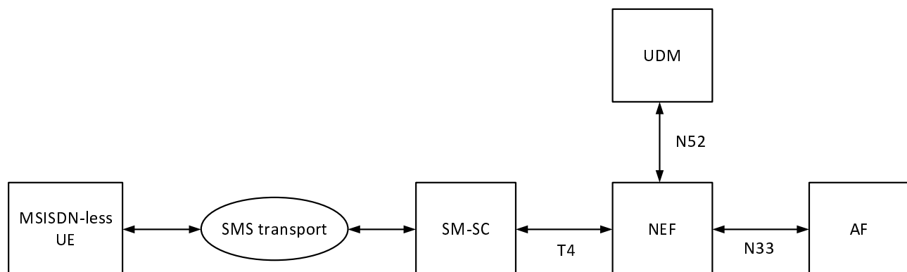
Figure 7.9-3: 5GS architecture for MSISDN-less MO SMS
