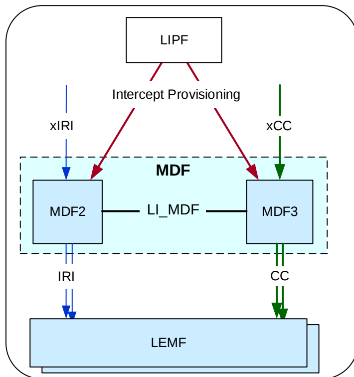
Figure 5.3-2: MDF2 and MDF3
