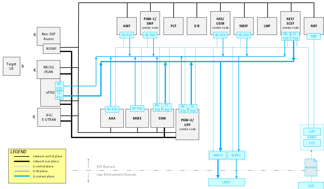
Figure 6.6-1: EPC/5G Interworking LI architecture
