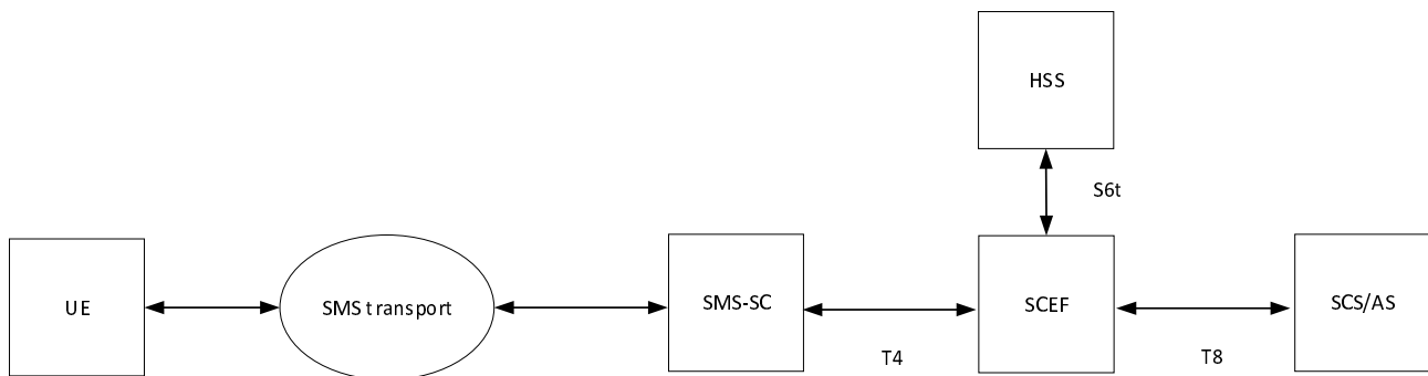
Figure 7.11-2: EPS architecture for device triggering
