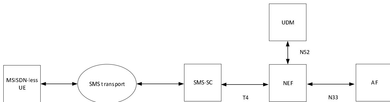
Figure 7.9-3: 5GS architecture for MSISDN-less MO SMS
