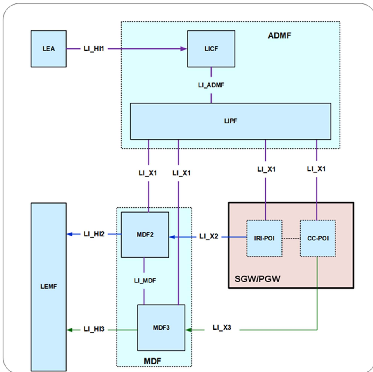
Figure 6.3-2: LI architecture for LI at non-CUPS SGW/PGW
