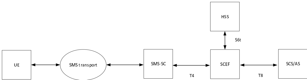
Figure 7.11-2: EPS architecture for device triggering
