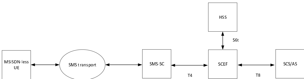
Figure 7.11-3: EPS architecture for MSISDN-less MO SMS
