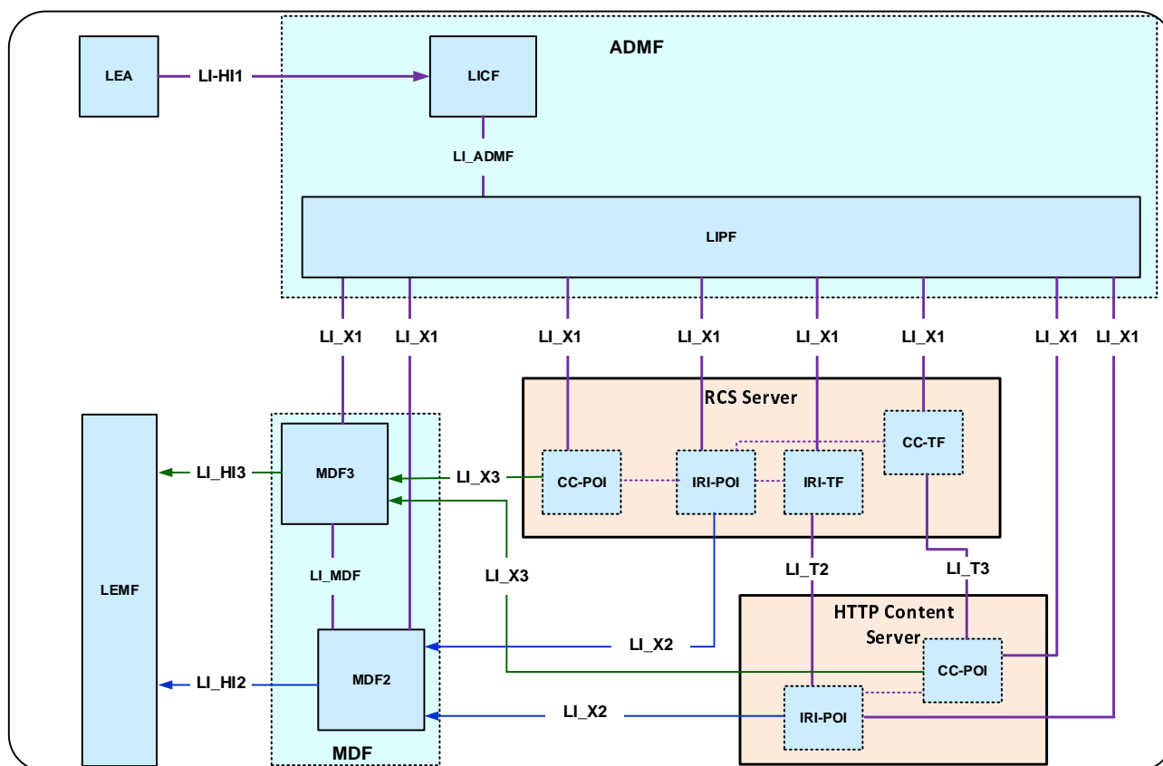
Figure 7.13.2-1: LI architecture for RCS services
