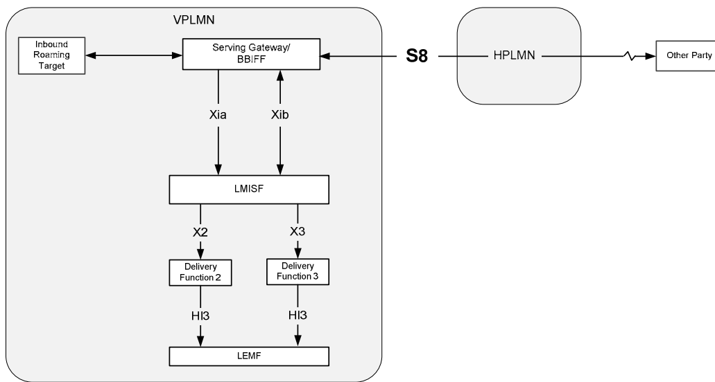
Figure 12.1: Lawful Interception in the VPLMN with S8HR as the roaming architecture
