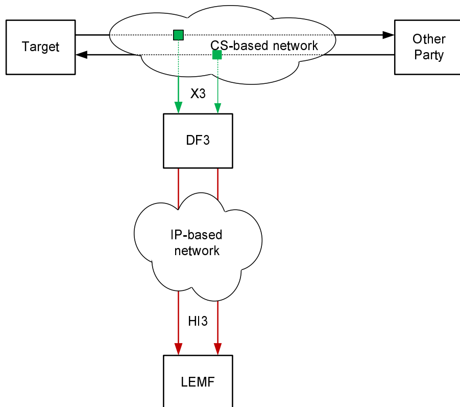
Figure 5.5: IP based handover interface for the CC of CS intercepts
