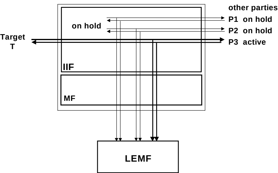
Figure 5.2: CC link option A (example for call hold supplementary service)
