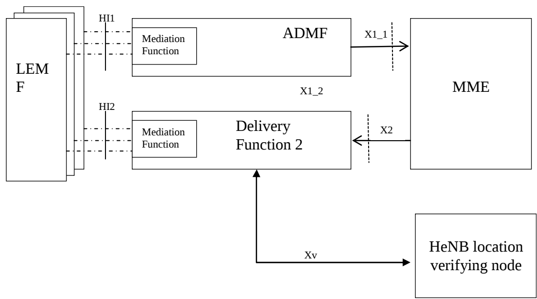
Figure 12.1.1a: Configuration for Intercept of HeNB
