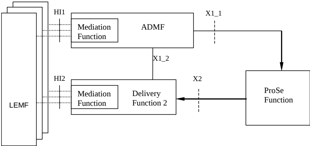
Figure 17.1-1: ProSe Direct Discovery Intercept configuration
