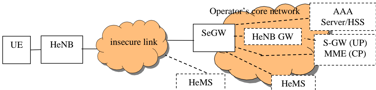
Figure 13-3: 3GPP HeNBs Architecture Basis for Lawful Interception
