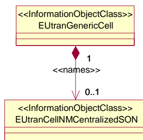
Figure 6.2.1.9: Cell SON Attributes NRM IOCs (Containment Relationship)
