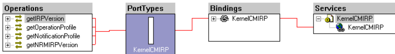
Figure C.3.2: kernelCM IRP SOAP Solution Set WSDL structure
