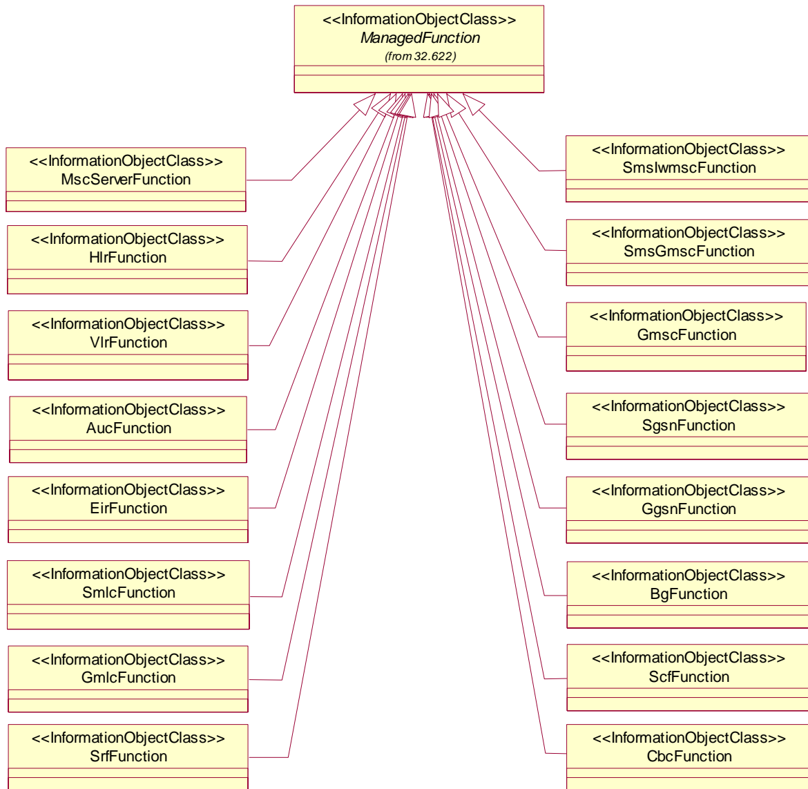
Figure 6.2.2.1: CN NRM Inheritance Hierarchy 1
