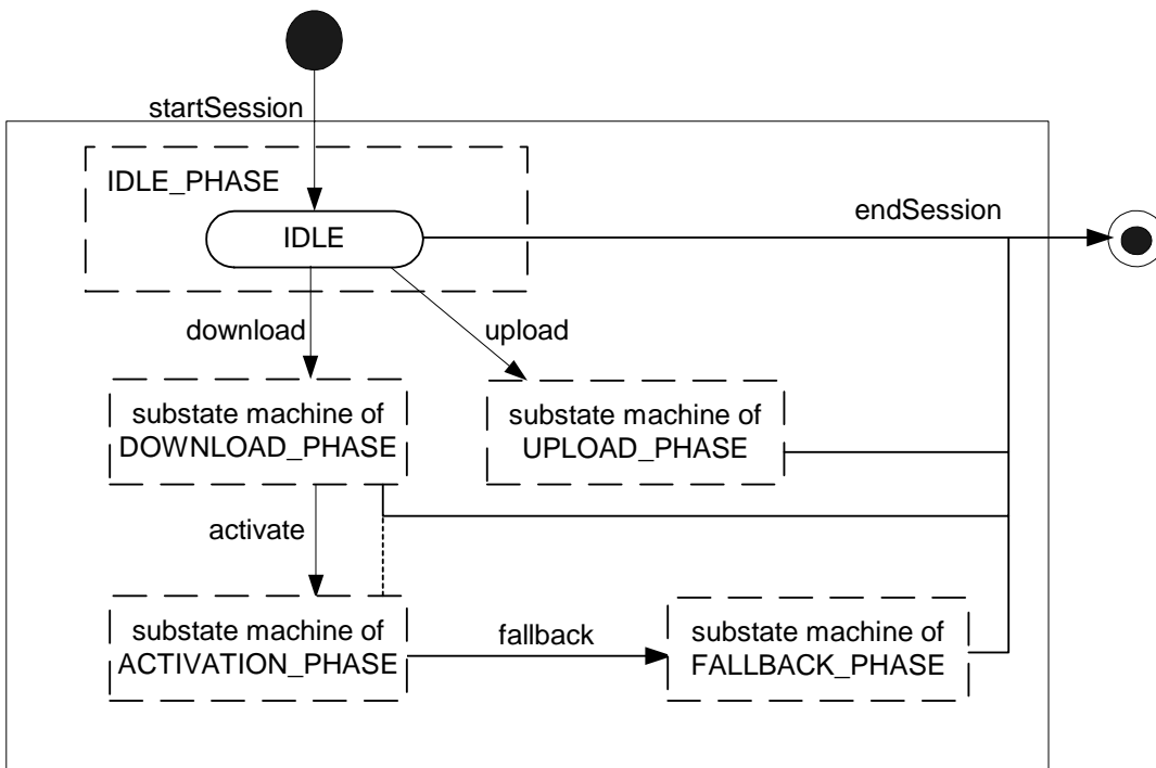
Figure 5: State Machine
