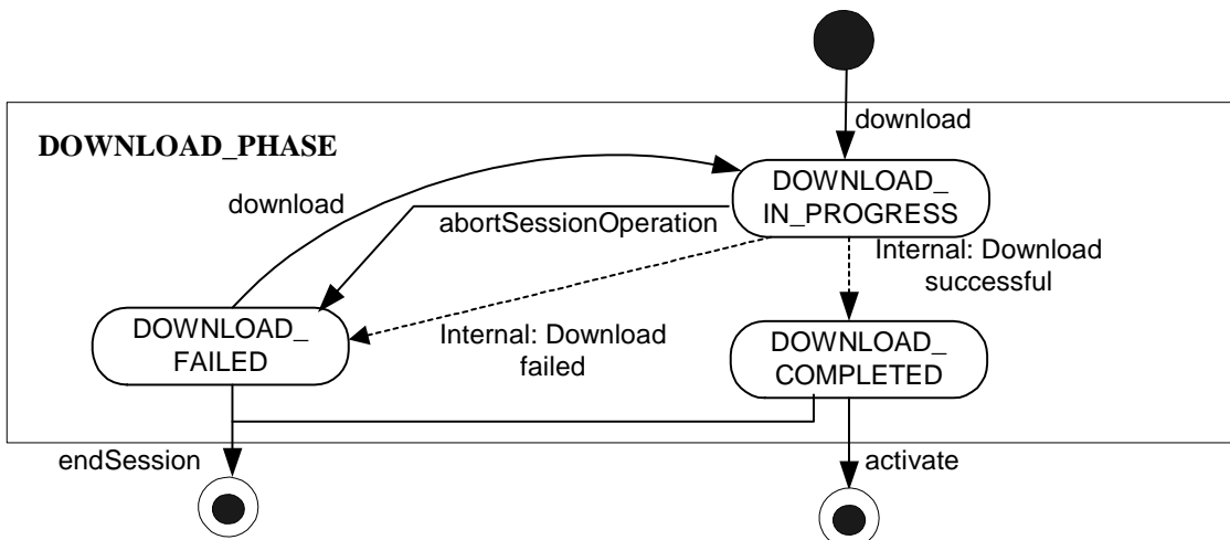
Figure 8: Substate Machine – DOWNLOAD_PHASE
