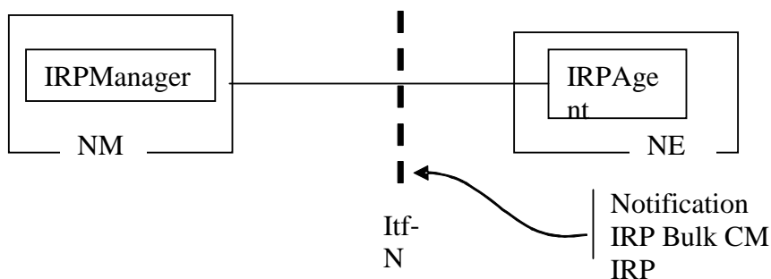
Figure 2: System Context A
