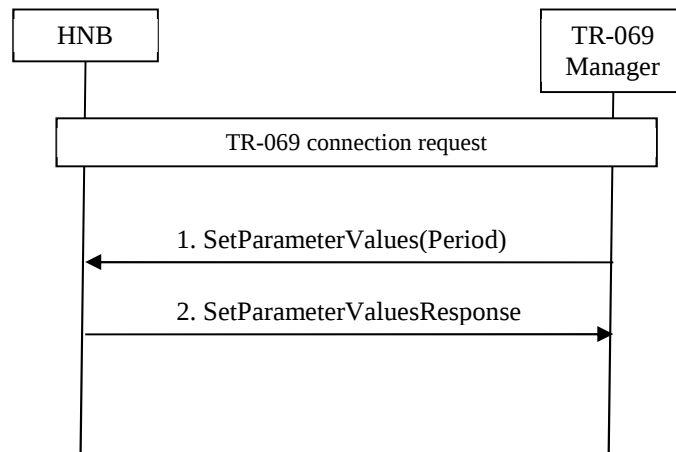
Figure 5.6.1-1: PM File Upload Period Set procedure flow
