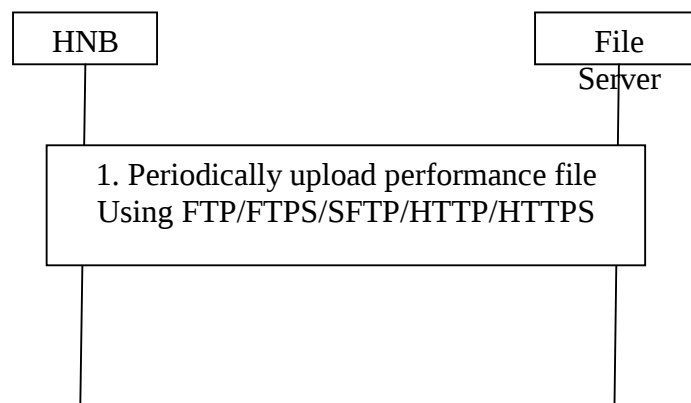
Figure 5.6.2-1: PM file uploading procedure flow
