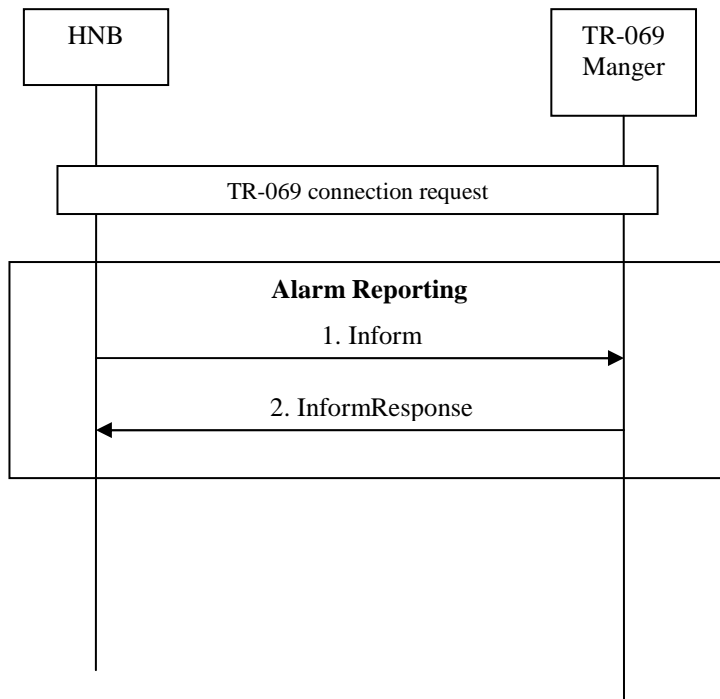
Figure 5.2.2-1: Alarm Reporting Procedure Flow
