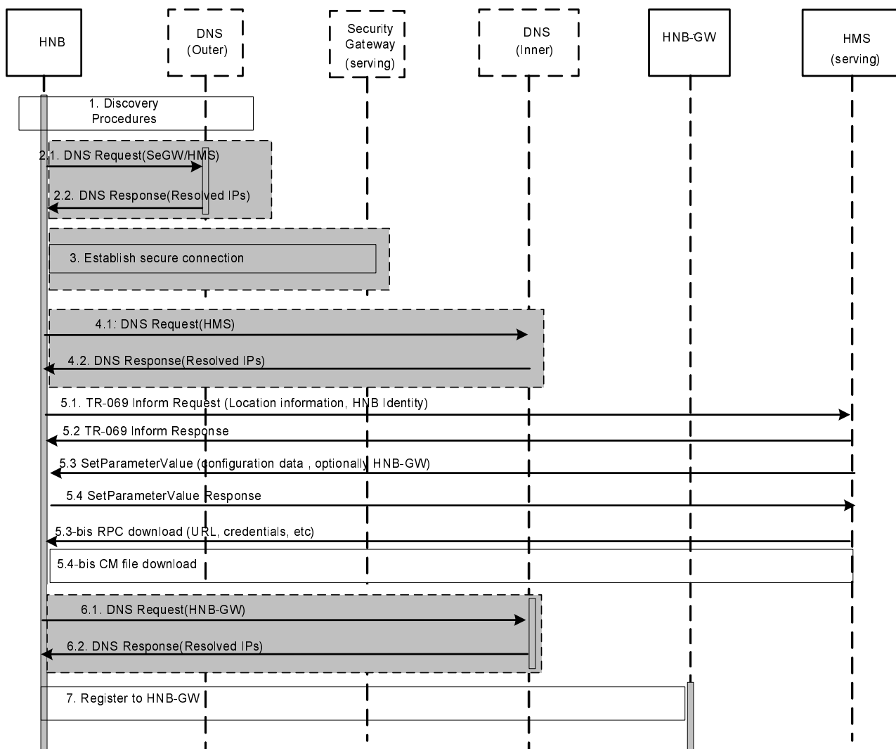
Figure 5.2.1-1: HNB Registration procedure flow
