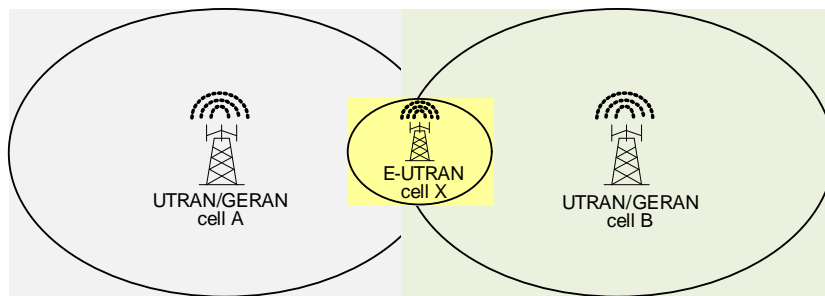
Figure B.5: E-UTRAN Cell overlaid by multiple UTRAN/GERAN Cells
