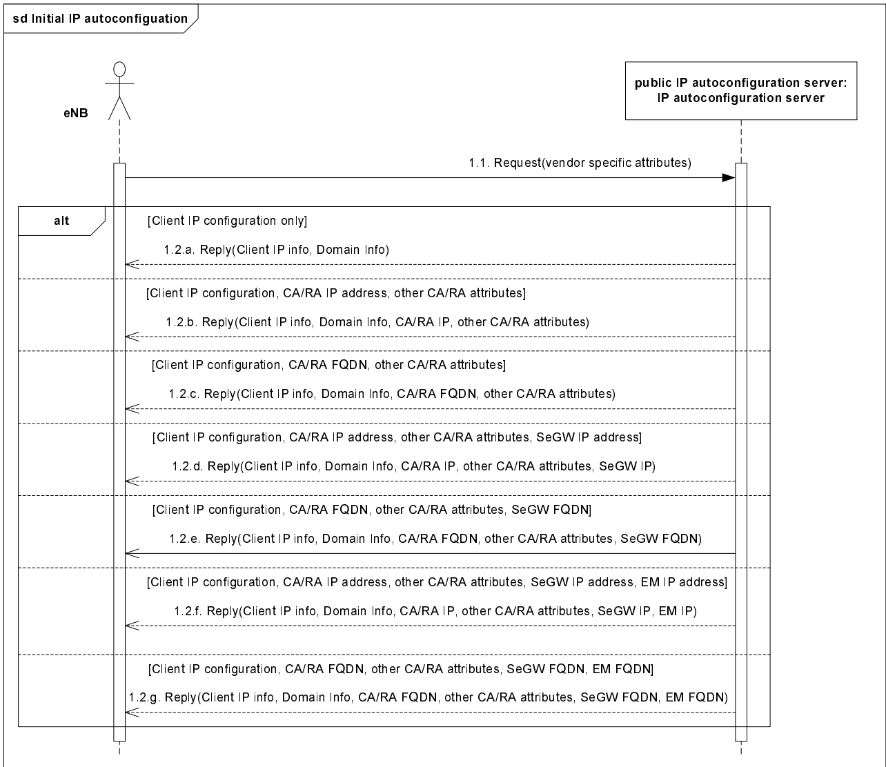
Figure 5.2-1: Initial IP Autoconfiguration flow
