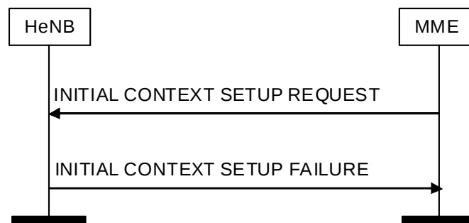
Figure 6 Initial Context Setup procedure. Unsuccessful operation
