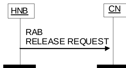
Figure 11 RAB Release Request procedure
