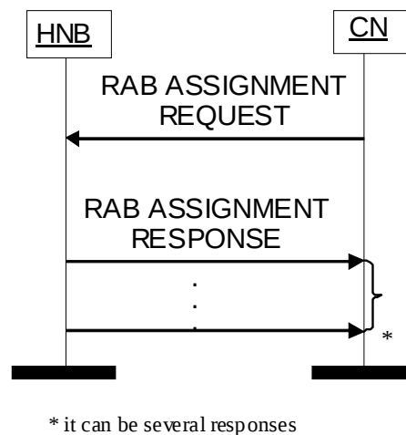
Figure 10 RAB Assignment procedure. Successful operation
