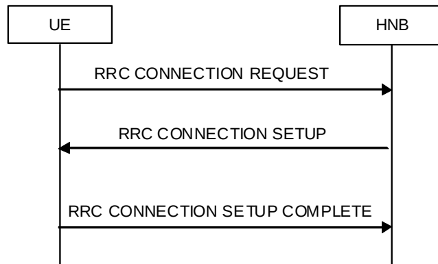
Figure 13 RRC Connection procedure, Successful operation
