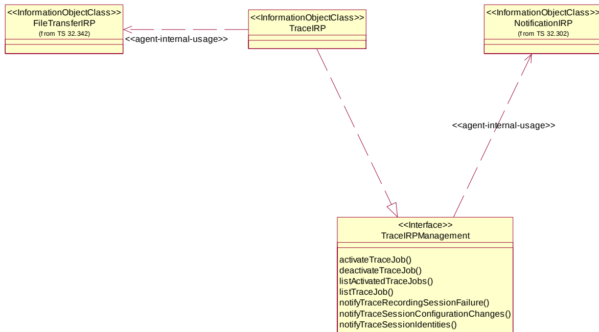
Figure 6.1: Class Diagram
